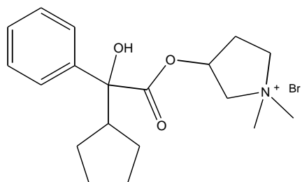
VIII. Glycopyrrolate [596-51-0]
