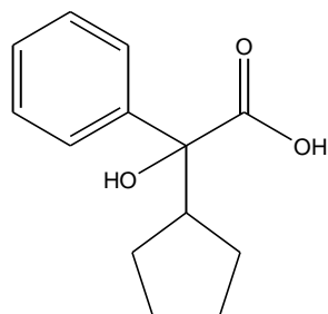
VII. Cyclopentyl Mandelic acid [427-49-6]
