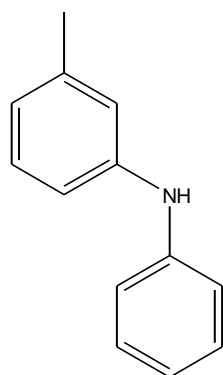
IX. 3-Methyldiphenyl amine [1205-64-7]
