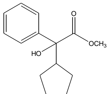
VIII. Cyclopentyl Mandelic acid, Methyl ester
